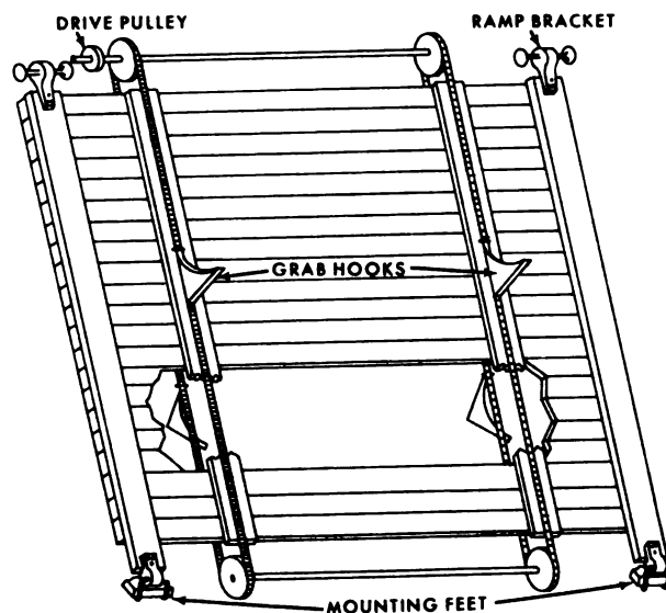
Figure 7-21. Jackladder.
